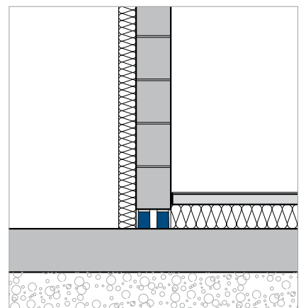
Application with insulation at the base of the wall on the base slab.
