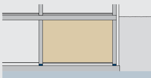
Laundry room / sauna: base slab solution
