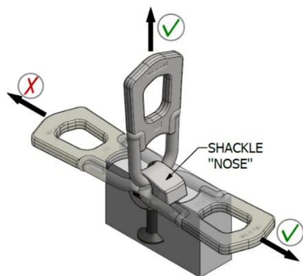
Angled lifting
