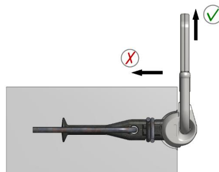
Tilt-up lifting
